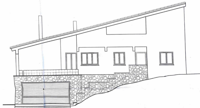
ALZADO PRINCIPAL
