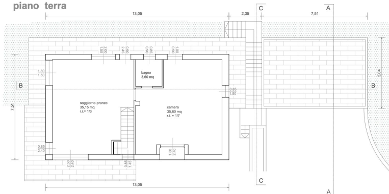
piano terra
