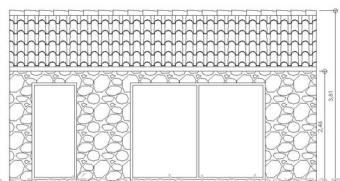
FACHADA PRINCIPAL I
